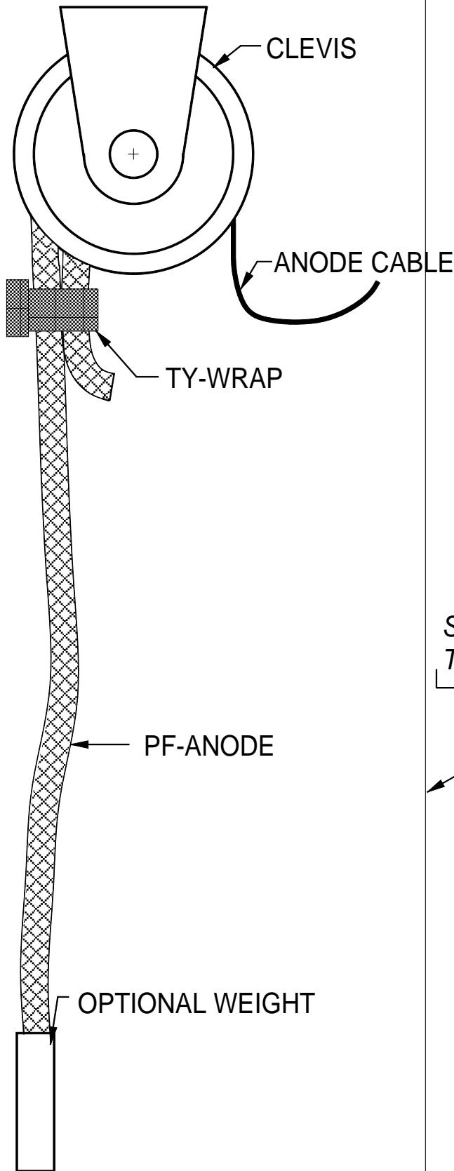
TYPICAL WATER TANK INSTALLATION
